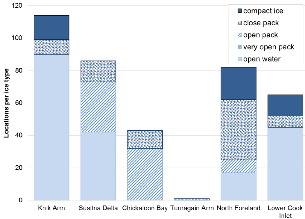
Figure 60. -- Ice associations for beluga CI-0105 tagged in Cook Inlet, Alaska, 13 August 2001. Histograms show number of modelled locations per day (top panel) and per region (bottom panel) in each ice type (see text for details). Note: "North Foreland" includes all waters south of North Foreland and Point Possession, and north of East and West Foreland.
