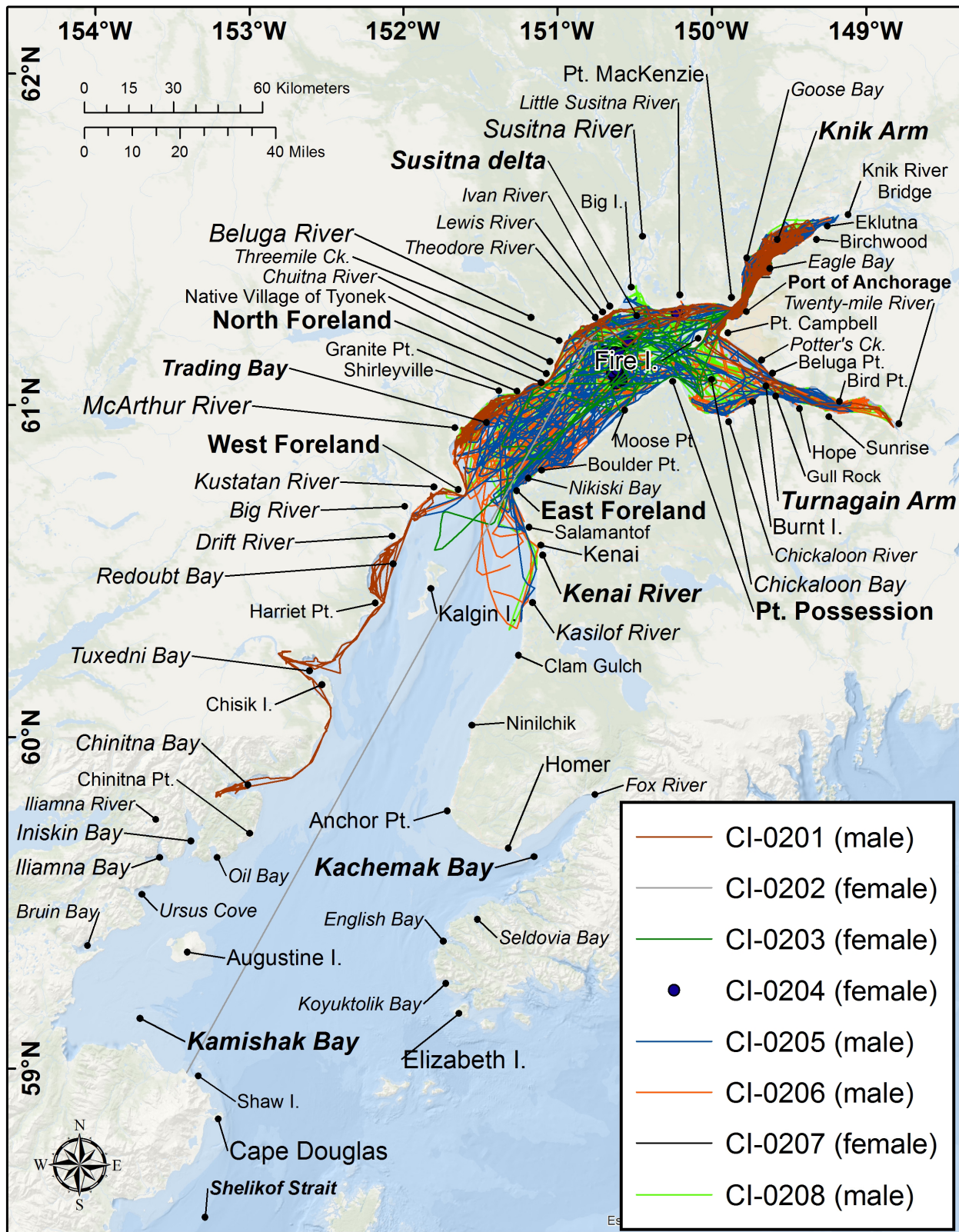
Figure 69. -- Satellite-linked modelled tracks from belugas tagged in Cook Inlet, Alaska, in late July and early August 2002. Tags attached to CI-0202 (female), CI-0204 (female), and CI-0207 (female) transmitted > 2 days post-tagging (see text).
