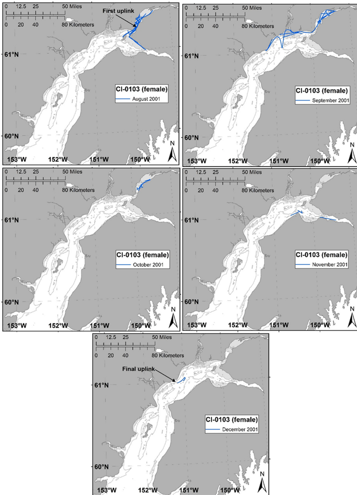
Figure 55. -- Monthly movement tracks (blue) of beluga CI-0103 tagged in Cook Inlet, Alaska, 12 August 2001. Note: the ST16 tag ceased transmitting on 30 Sept., the first transmission from the SPOT2 occurred on 29 September.
