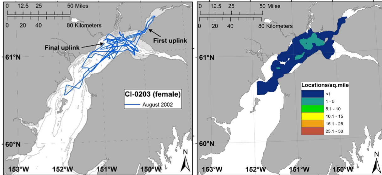
Figure 75. -- Monthly movement tracks (blue) and density (low to high kernel of modelled locations per sq. mile) of beluga CI-0203 tagged in Cook Inlet, Alaska, 31 July 2002.
