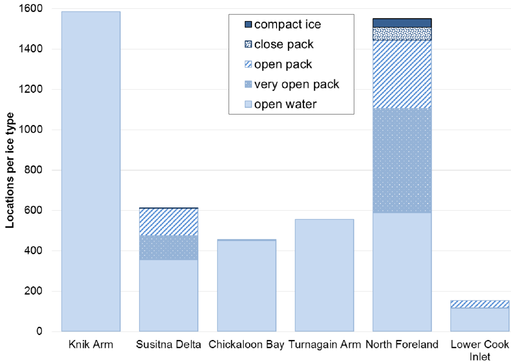
Figure 84. -- Ice associations for beluga CI-0206 tagged in Cook Inlet, Alaska, 3 August 2002. Histograms show number of modelled locations per day (top panel) and per region (bottom panel) for each ice type (see text for details). Note: "North Foreland" includes all waters south of North Foreland and Point Possession, and north of East and West Foreland.
