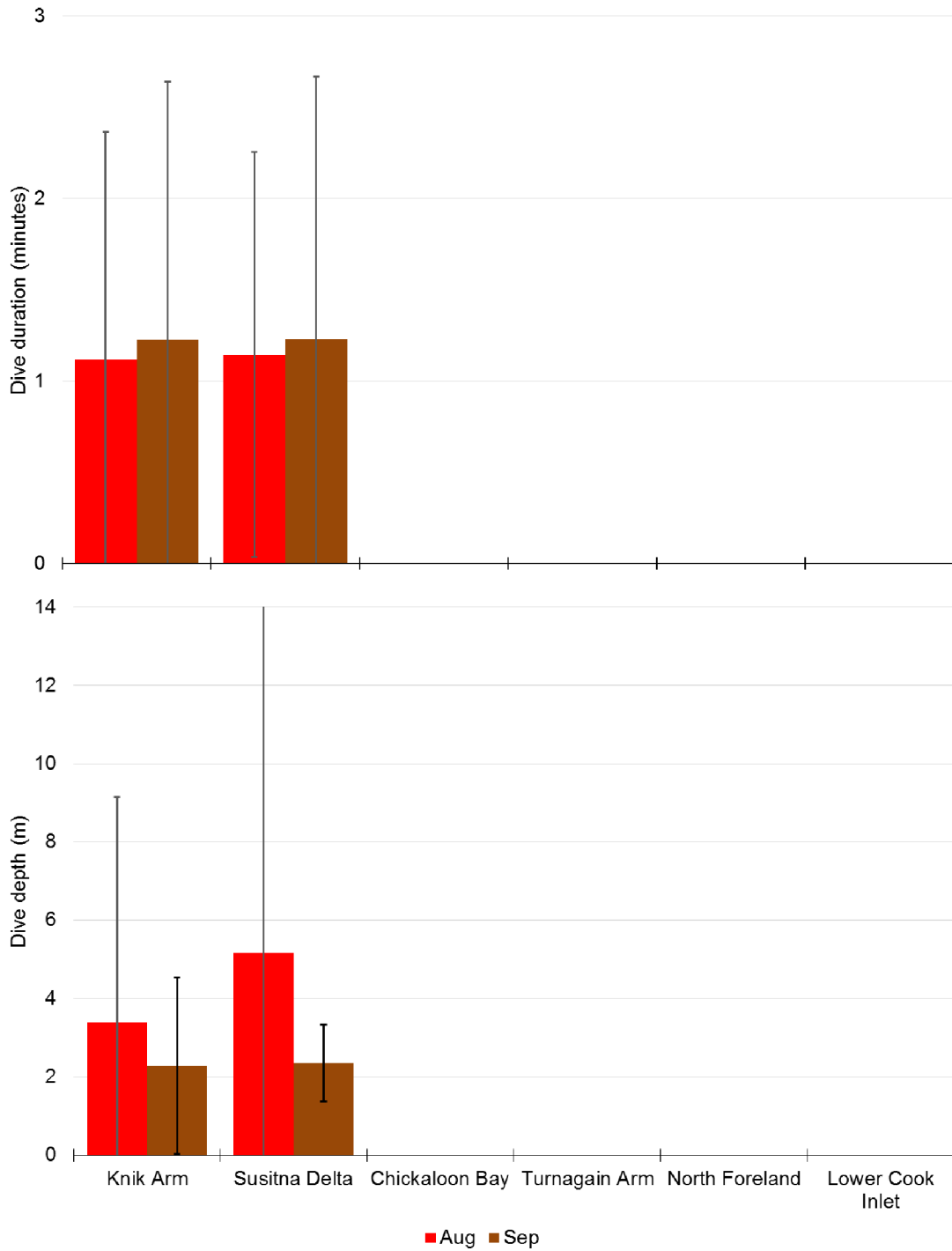
Figure 57. -- Monthly dive behavior of beluga CI-0103 tagged in Cook Inlet, Alaska, 12 August 2001. Histograms show average dive duration in minutes (top panel) and average dive depth in meters (bottom panel) for binned data (see Table 1) within specific regions of the inlet for each month (SD = error bars). Note: "North Foreland" includes all waters south of North Foreland and Point Possession, and north of East and West Foreland.
