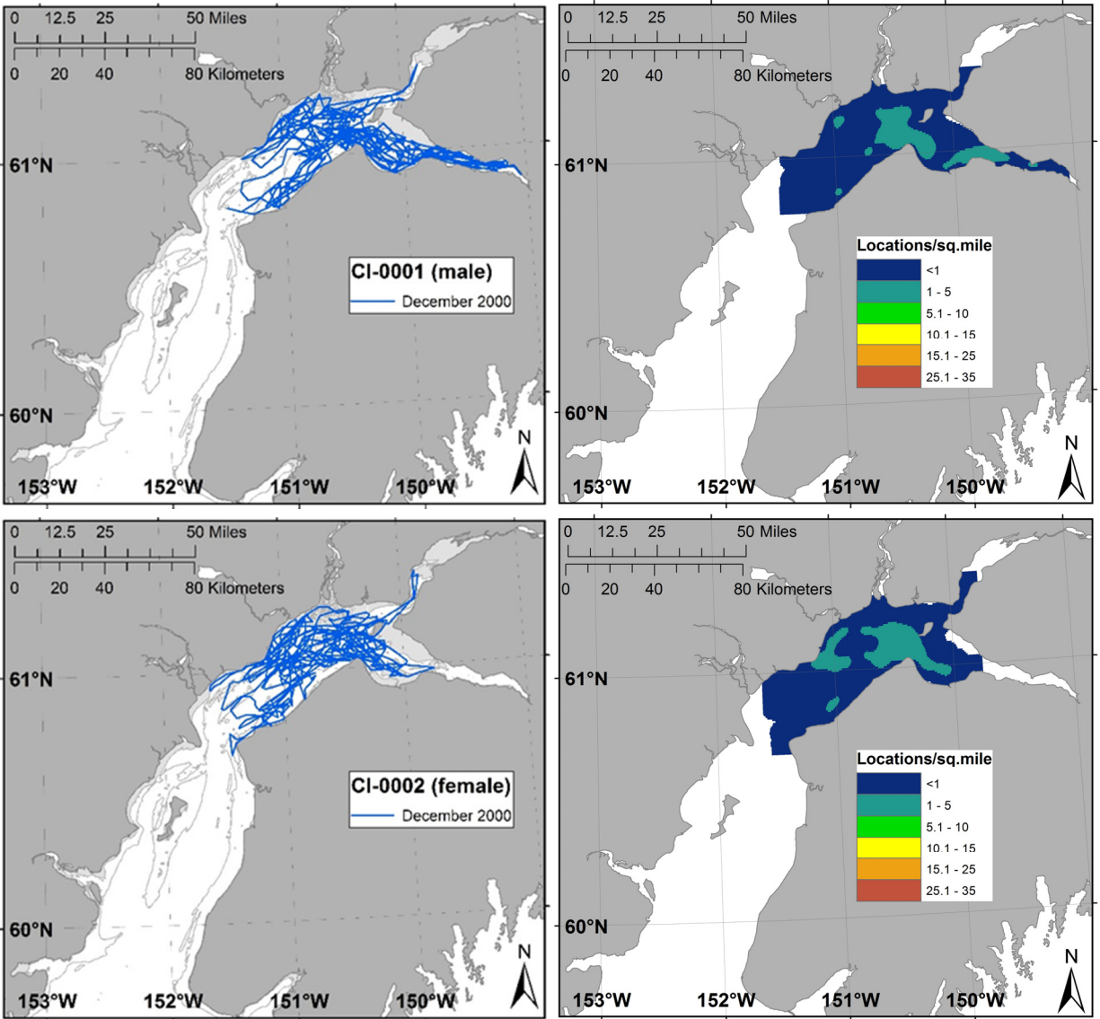
Figure 40. -- Monthly movement tracks (blue) and density (low to high kernel of modelled locations per sq. mile) of belugas CI-0001 and CI-0002 in Cook Inlet, Alaska, in December 2000.
