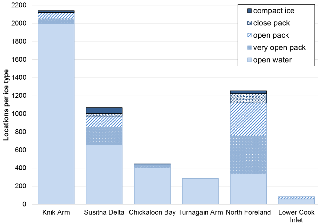
Figure 80. -- Ice associations for beluga CI-0205 tagged in Cook Inlet, Alaska, 2 August 2002. Histograms show number of modelled locations per day (top panel) and per region (bottom panel) for each ice type (see text for details). Note: "North Foreland" includes all waters south of North Foreland and Point Possession, and north of East and West Foreland.
