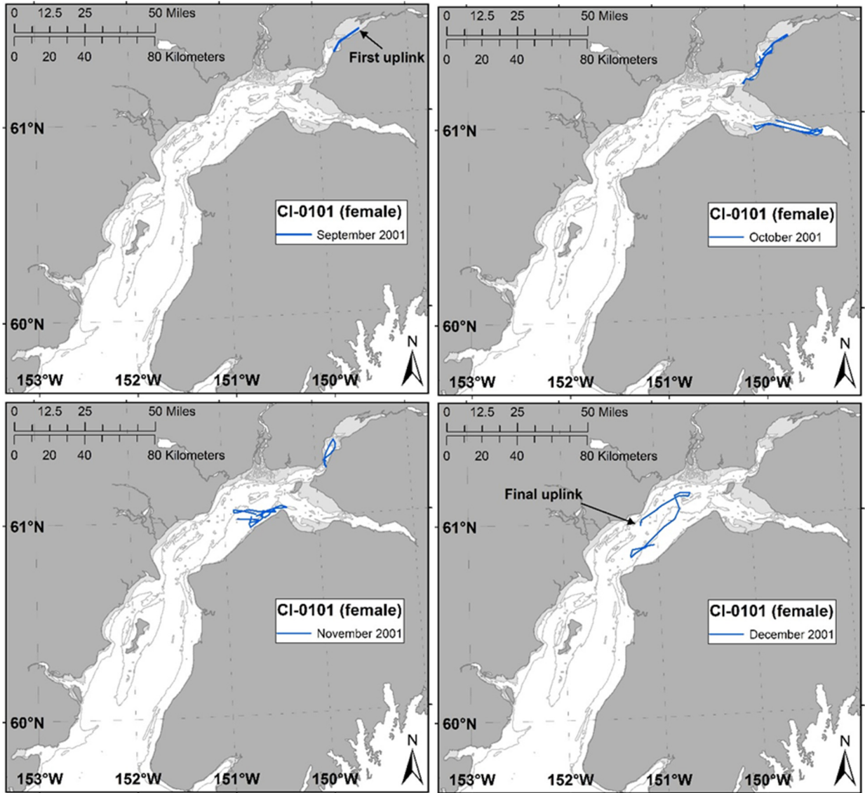
Figure 49. -- Monthly movement tracks (blue) of beluga CI-0101 tagged in Cook Inlet, Alaska, 10 August 2001. Note: SPOT2 tag was duty cycled to transmit only 3 days per month.
