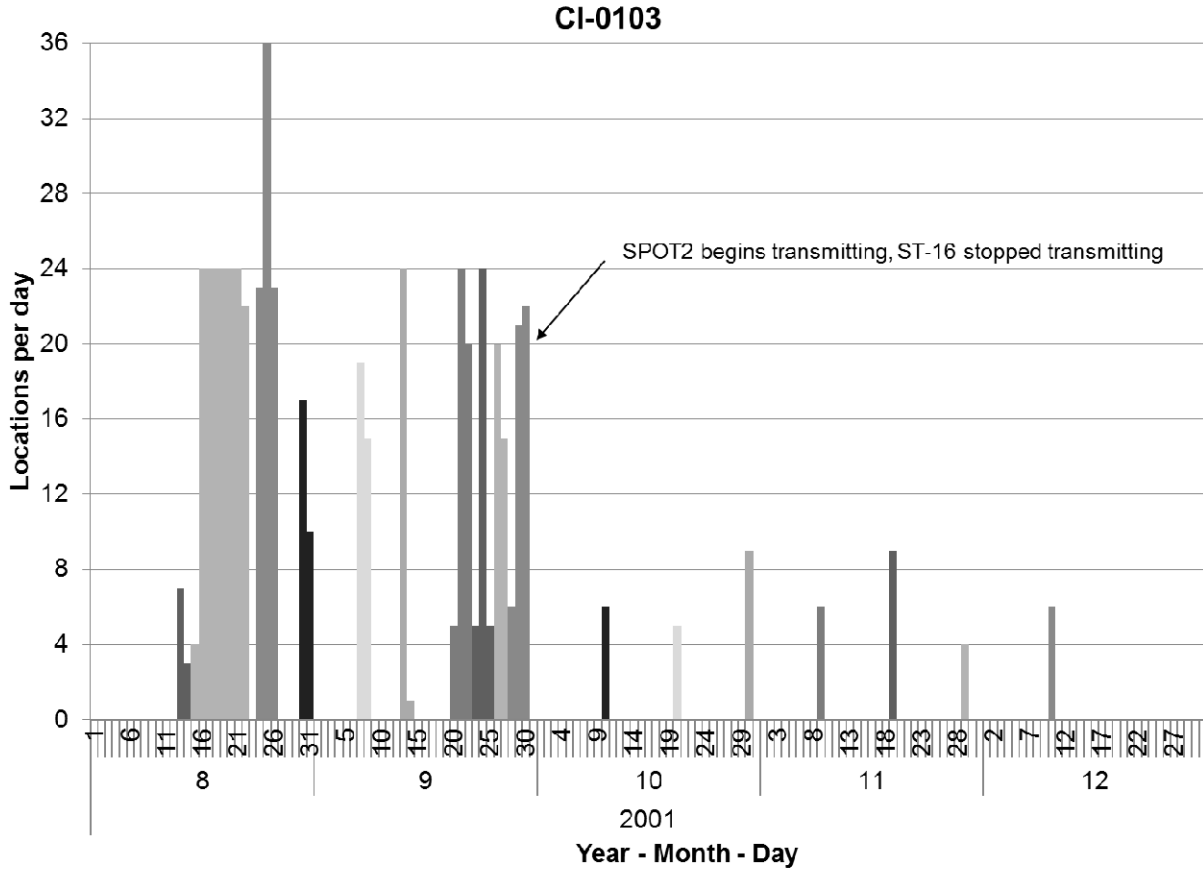
Figure 54. -- Number of modelled locations for satellite-linked transmissions from beluga CI-0103 tagged in Cook Inlet, Alaska, 12 August 2001. The ST16 was programmed to transmit daily but gaps in transmissions began occurring during August and no status updates were received from this tag. Transmissions and temperature readings from the SPOT2 were expected to occur 3 days per month (9 th , 19 th , and 29 th ) for 24 hours, but no TAT data were transmitted (Appendix 11). A change in column color denotes transmission gaps > 1 day. Transmissions were received from mid-August 2001 into December 2001 (covering a 130-day period with 21.8 days of data usable for analysis).
