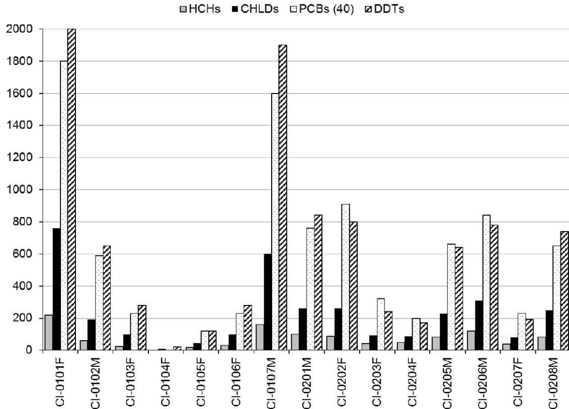
Figure 28. -- Concentrations of \Sigma HCHs, \Sigma CHLDs, \Sigma PCBs, and \Sigma DDTs (ng/g, wet weight) determined by gas chromatography/mass spectrometry for belugas tagged in 2001 and 2002 (methods in Krahn et al. 2004). See Appendix 4 for values.
